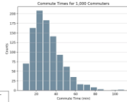
A histogram
