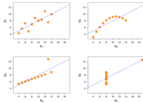
Anscombe's quartet
