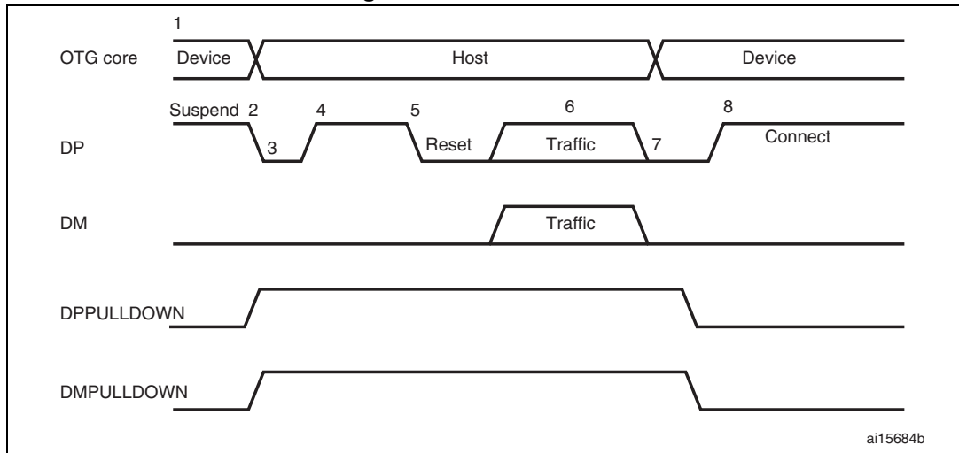
Figure 433. B-device HNP
