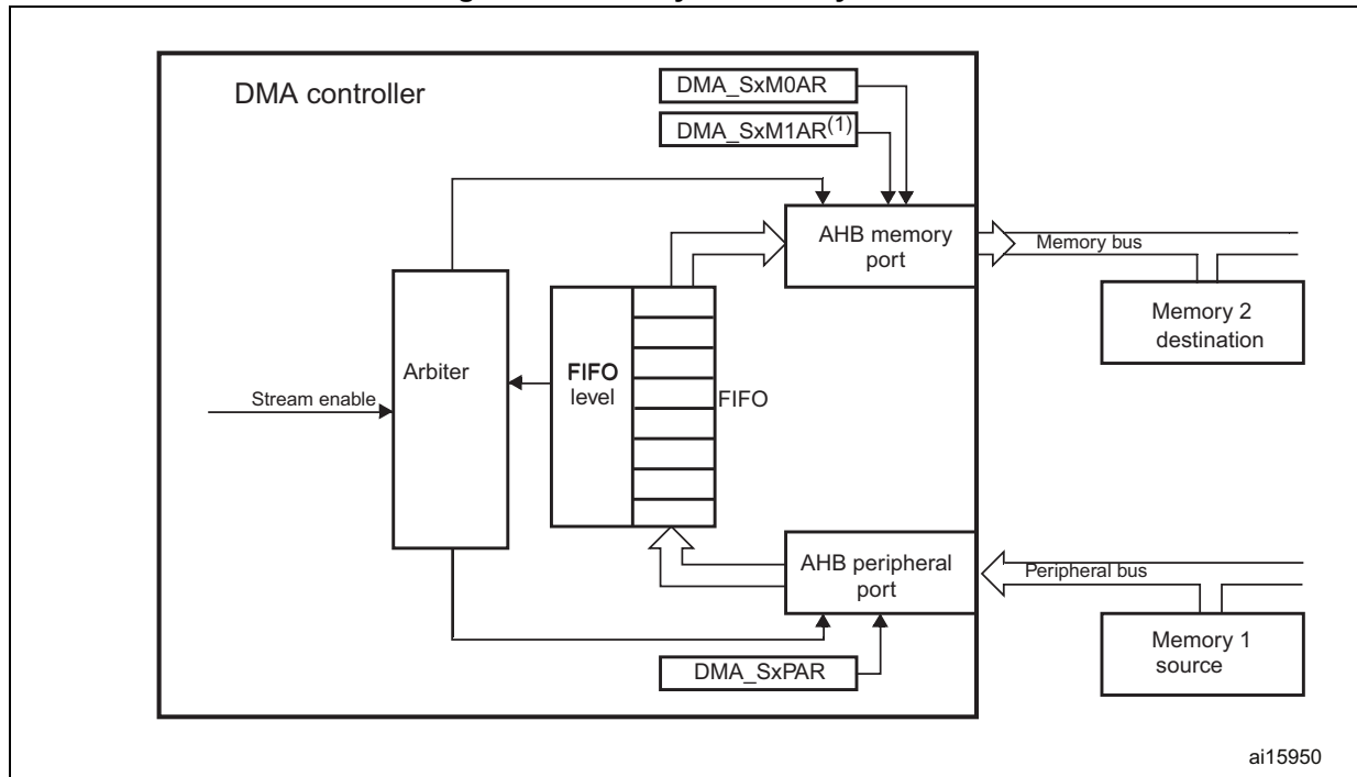
Figure 38. Memory-to-memory mode
