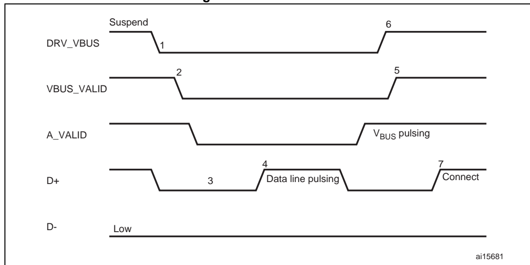
Figure 406. A-device SRP
