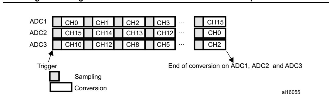
Figure 55. Regular simultaneous mode on 16 channels: triple ADC mode
