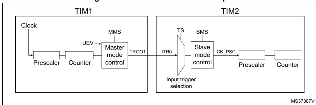
Figure 174. Master/Slave timer example
