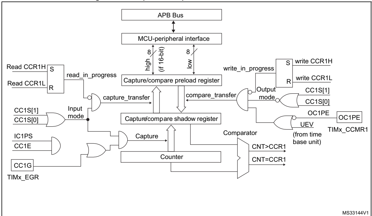
Figure 160. Capture/compare channel 1 main circuit
