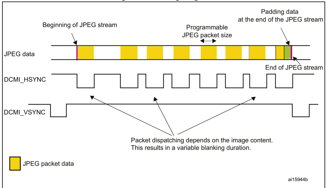
Figure 75. Timing diagram
