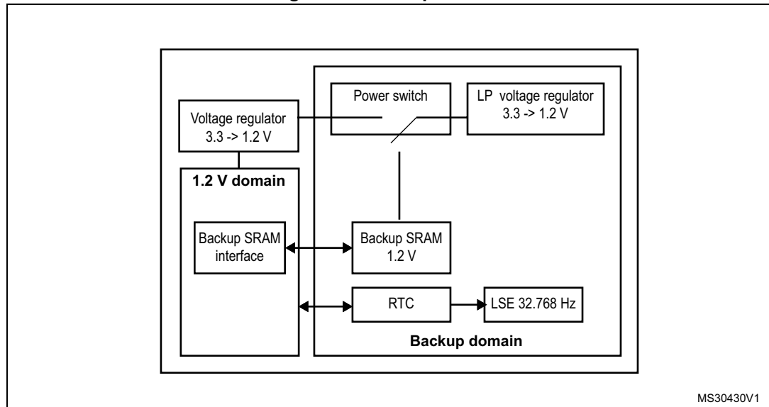
Figure 11. Backup domain
