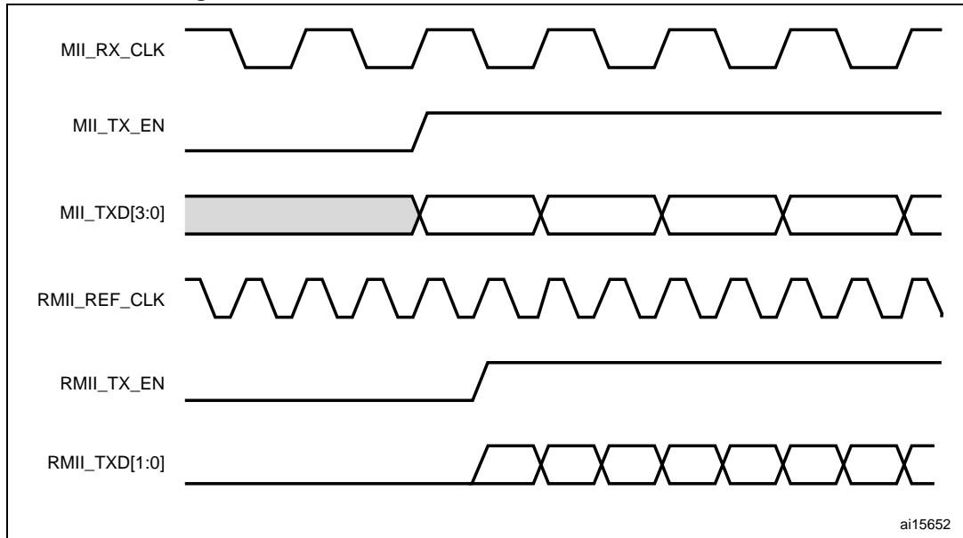
Figure 365. Frame transmission in MMI and RMII modes
