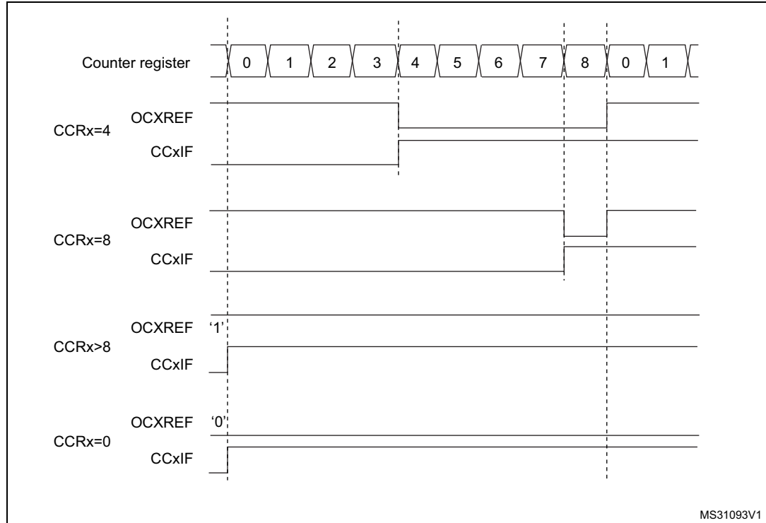
Figure 198. Edge-aligned PWM waveforms (ARR=8)
