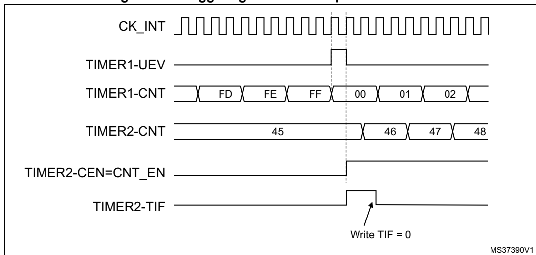
Figure 177. Triggering timer 2 with update of timer 1
