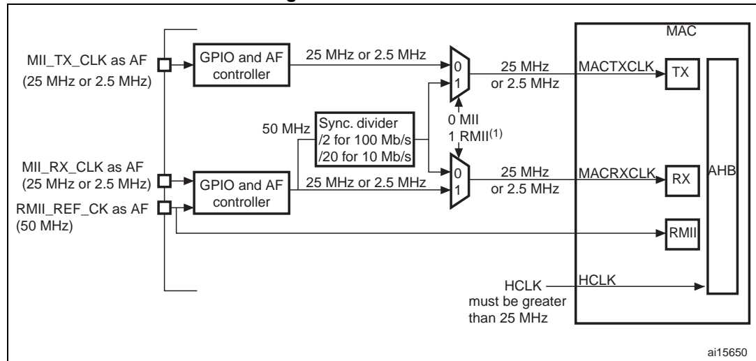
Figure 358. Clock scheme
