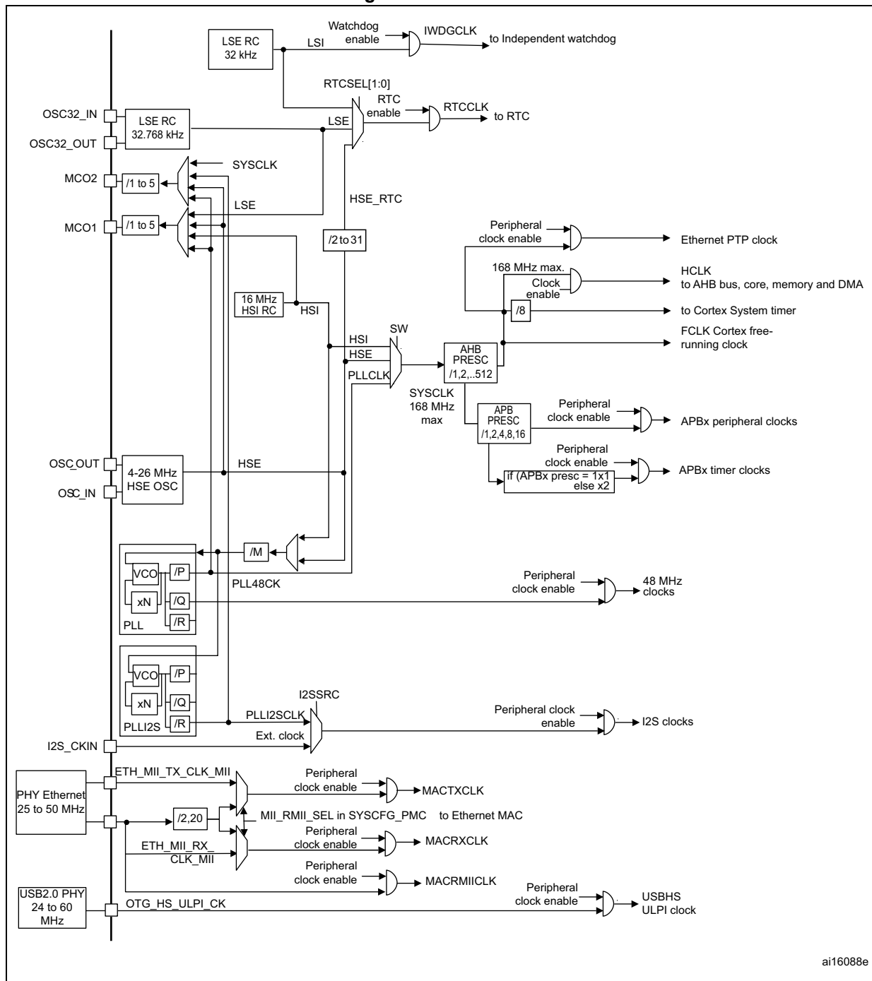
Figure 21. Clock tree
